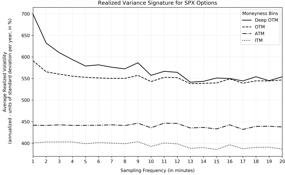
Figure 1: The figure shows the average realized volatility (annualized in percentage) for options of different moneyness. The realized volatilities are computed using different sampling frequencies. The sampling frequency varies from 1-minute up to 20-minutes. Higher sampling frequencies are at the left side of the figure, while lower sampling frequencies are at the right side of the figure. The realized volatility is estimated as the sum of squared returns over each day for each option. The figure shows an increase in the volatility for out-of-the-money options when the sampling frequency is below 5-minutes, indicating the presence of microstructure noise.
