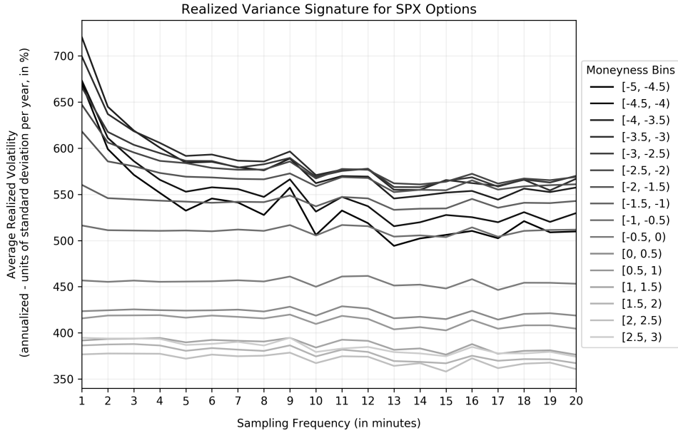
Figure 5: The figure shows the average realized volatility (annualized in percentage) for options of different moneyness. The realized volatilities are computed using different sampling frequencies. The sampling frequency varies from 1-minute up to 20-minutes. Higher sampling frequencies are at the left side of the figure, while lower sampling frequencies are at the right side of the figure. The realized volatility is estimated as the sum of squared returns over each day for each option.
