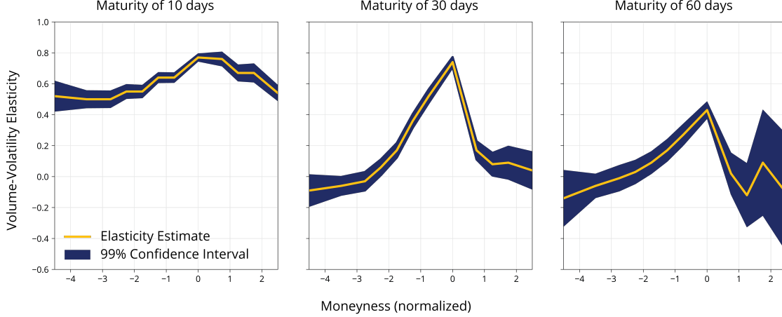
Figure 3: The figure reports volume-volatility elasticity estimates based on a nonparametric procedure (regressions group by group). Options are grouped by moneyiness and tenor in order to obtain the estimates. The estimates are based on the full sample of cleaned data, spanning 2007 to 2016. Moneyiness is measured in units of standard deviation and tenor is measured in days. Lines (yellow) display the elasticity estimates, while the shaded regions (blue) are 99% confidence intervals. Confidence intervals are computed using cluster-robust standard errors as in Petersen (2009). Each plot displays the volume-volatility elasticity as a function of moneyiness, while maintaining a fixed tenor.
