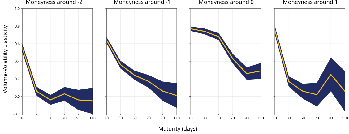
Figure 4: The figure reports volume-volatility elasticity estimates based on a nonparametric procedure (regressions group by group). Options are grouped by moneyness and tenor in order to obtain the estimates. The estimates are based on the full sample of cleaned data, spanning 2007 to 2016. Moneyness is measured in units of standard deviation and tenor is measured in days. Lines (yellow) display the elasticity estimates, while the shaded regions (blue) are 99% confidence intervals. Confidence intervals are computed using cluster-robust standard errors as in Petersen (2009). Each plot displays the volume-volatility elasticity as a function of tenor, while maintaining a fixed moneyness.
