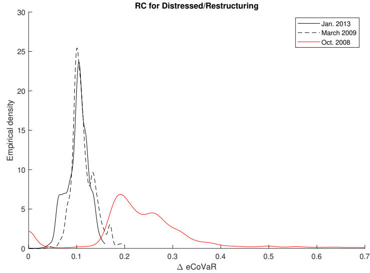
Figure 7: Empirical density of \Delta eCoVaR_\alpha^{k|l, \tilde{\alpha}} given by (18), with Distressed/Restructuring as a reference investment style. We fix \alpha = \tilde{\alpha} = .975 and use three different dates: October 2008 (red), March 2009 (dashed black), and January 2013 (solid black).
