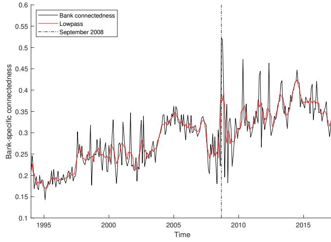
Figure 9: Black: \tilde{\chi}_t^{banks} (bank-specific connectedness). Red: lowpass moving average filter.
